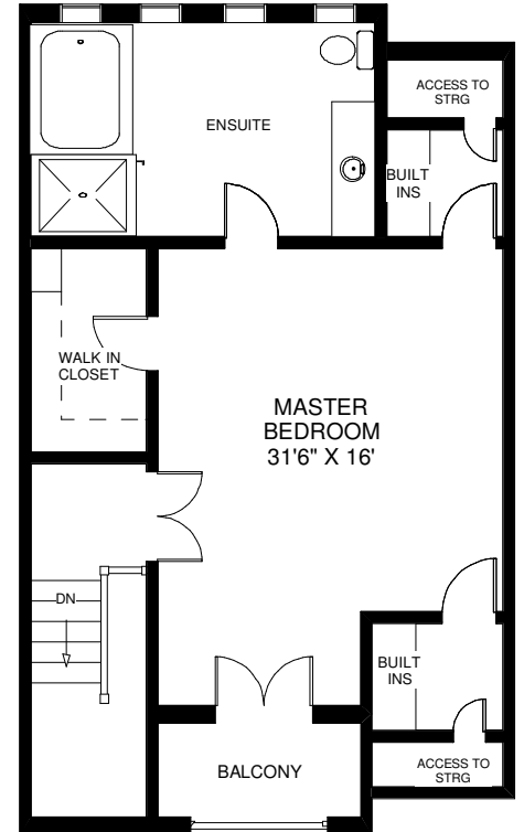
CEILING HT 9' THIRD FLOOR APPROXIMATELY 800 SQ FT
