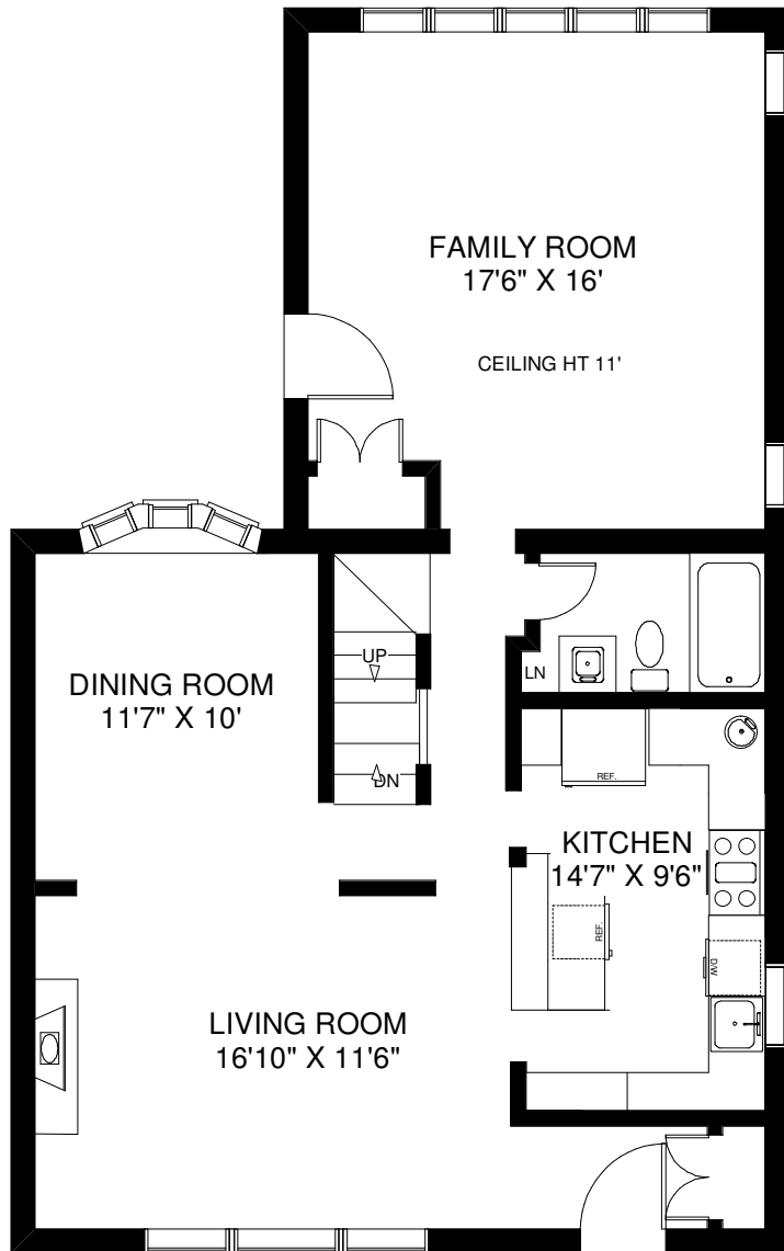
MAIN FLOOR APPROXIMATELY 1,060 SQ FT
