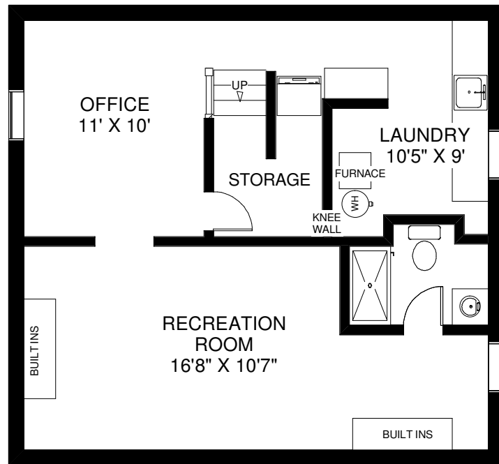
LOWER FLOOR APPROXIMATELY 720 SQ FT
