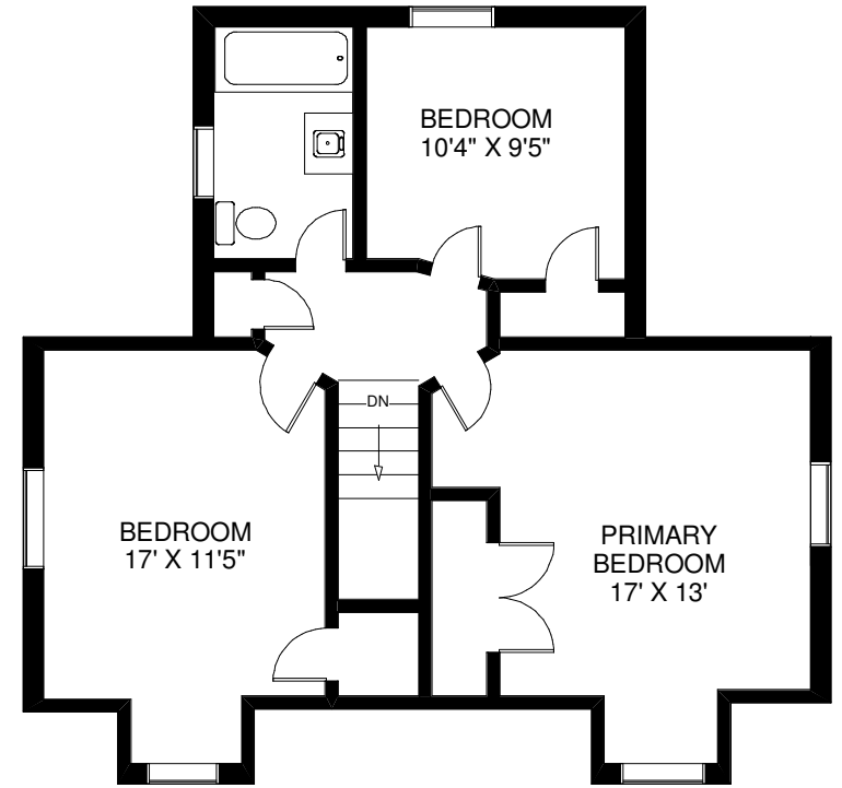
SECOND FLOOR APPROXIMATELY 800 SQ FT
