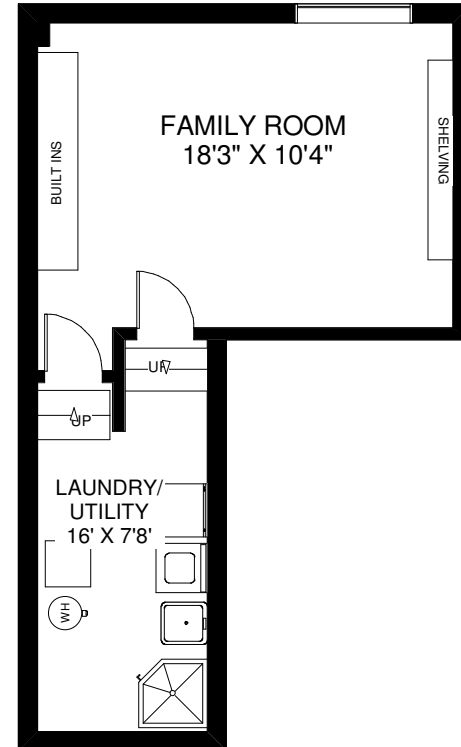
LOWER FLOORS APPROXIMATELY 460 SQ FT
