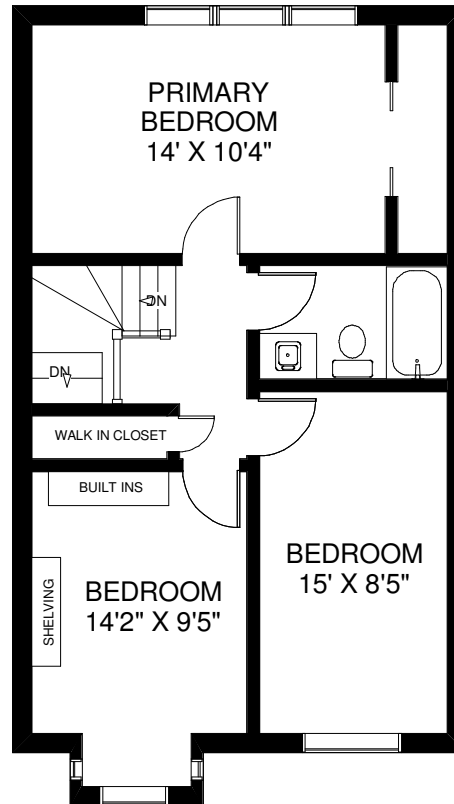
THIRD FLOOR APPROXIMATELY 650 SQ FT
