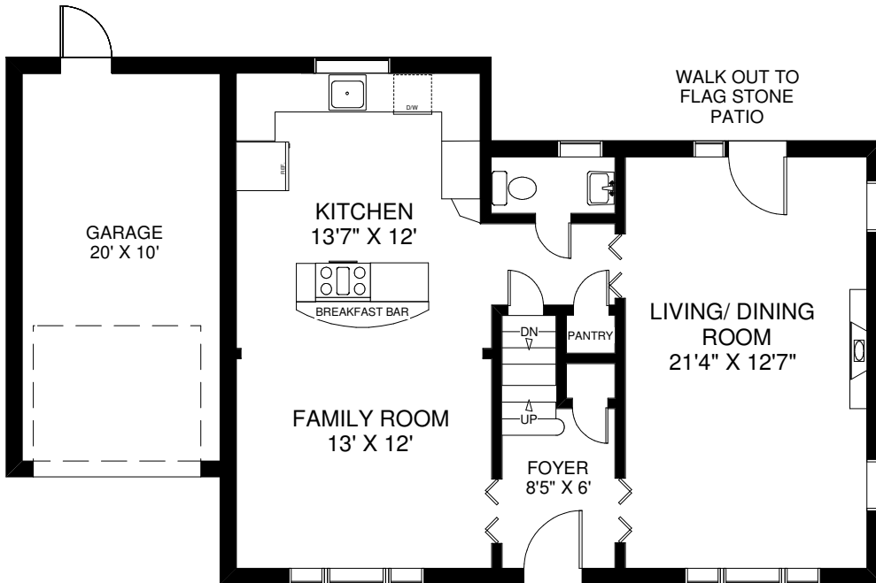
CEILING HT 8' MAIN FLOOR APPROXIMATELY 850 SQ FT
