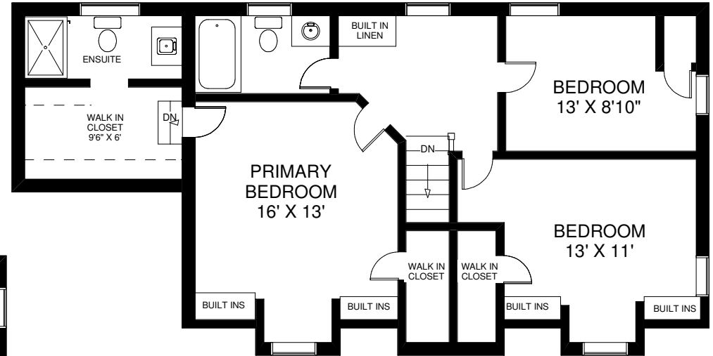
CEILING HT 8' SECOND FLOOR APPROXIMATELY 900 SQ FT
